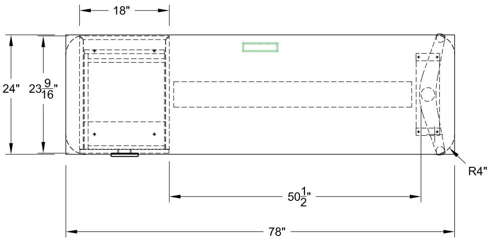
MDL: 42564/F (RECTANGLE) 42544/F (SOFT RECTANGLE) SIZE: 24" X 78"
