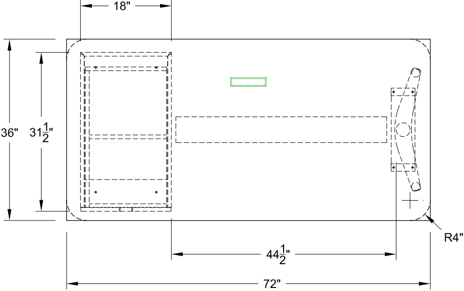
MDL: 42574/F (RECTANGLE) 42554/F (SOFT RECTANGLE) SIZE: 36" X 72"
