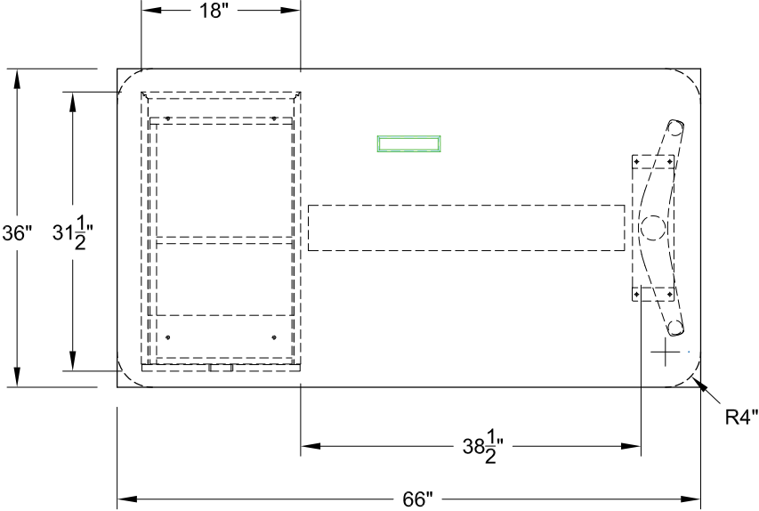
MDL: 42574/F (RECTANGLE) 42554/F (SOFT RECTANGLE) SIZE: 36" X 66"
