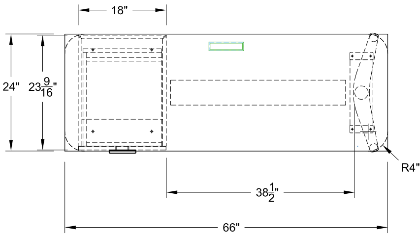
MDL: 42562/F (RECTANGLE) 42542/F (SOFT RECTANGLE) SIZE: 24" X 66"
