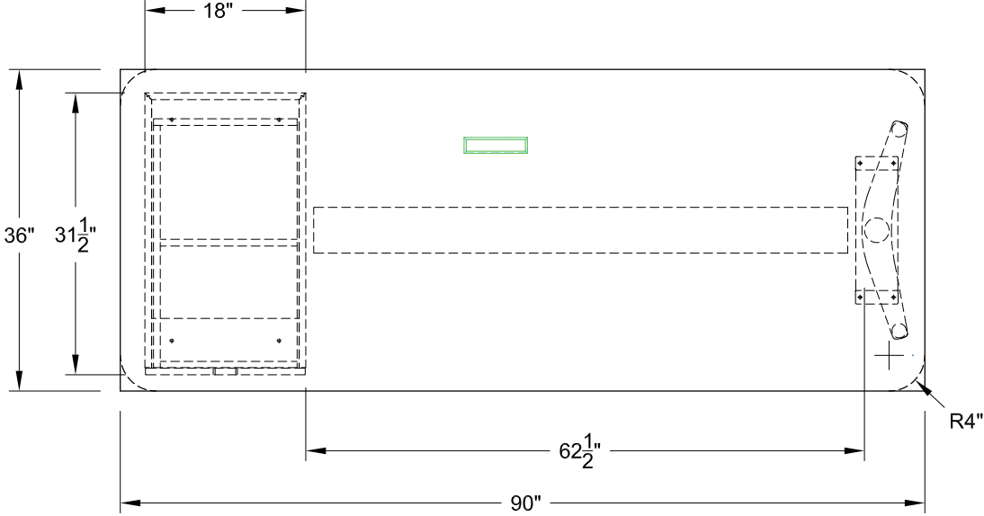
MDL: 42577/F (RECTANGLE) 42557/F (SOFT RECTANGLE) SIZE: 36" X 90"
