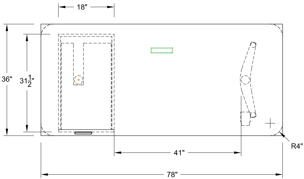
MDL: 42536/A (RECTANGLE) 42516/A (SOFT RECTANGLE) SIZE: 36" X 78"
