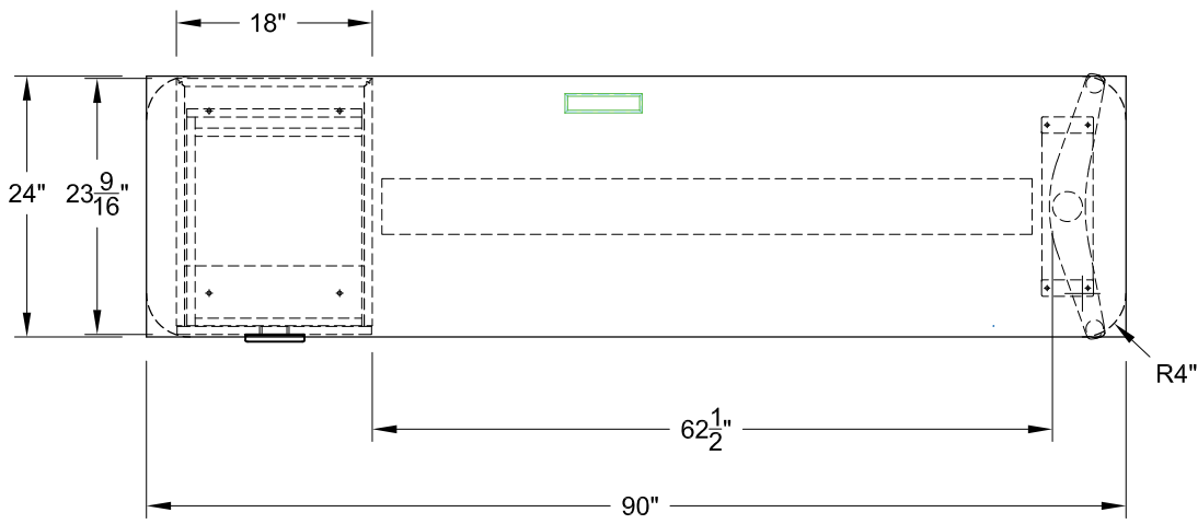
MDL: 42566/F (RECTANGLE) 42546/F (SOFT RECTANGLE) SIZE: 24" X 90"
