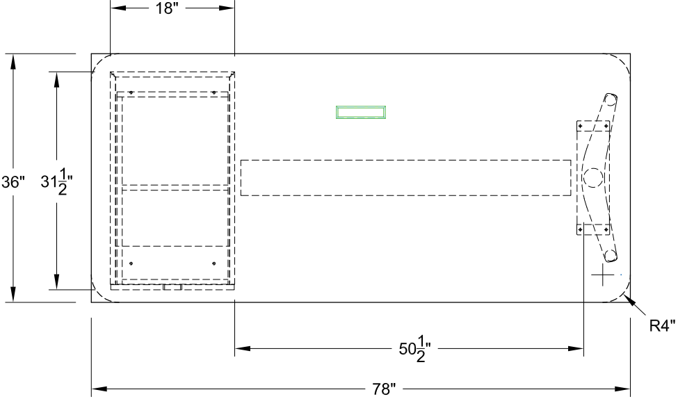
MDL: 42575/F (RECTANGLE) 42555/F (SOFT RECTANGLE) SIZE: 36" X 78"
