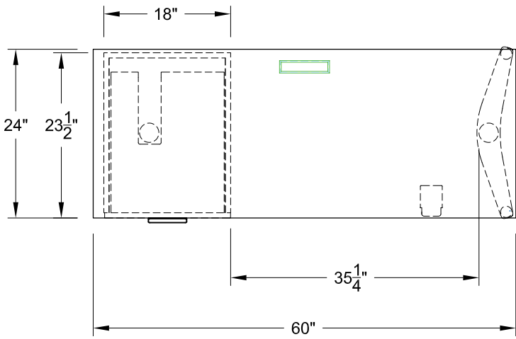
MDL: 42521/A (RECTANGLE) SOFT CORNERS NOT AVAILABLE SIZE: 24" X 60"
