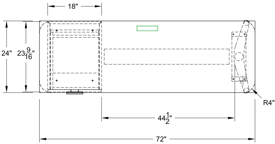
MDL: 42563/F (RECTANGLE) 42543/F (SOFT RECTANGLE) SIZE: 24" X 72"
