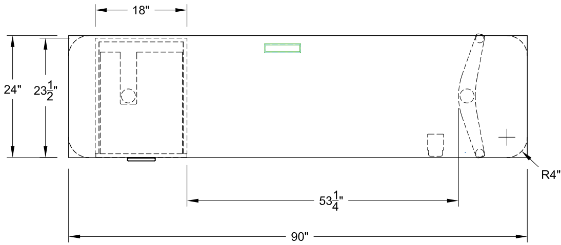
MDL: 42526/A (RECTANGLE) 42506/A (SOFT RECTANGLE) SIZE: 24" X 90"
