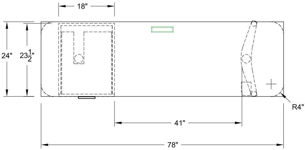
MDL: 42524/A (RECTANGLE) 42504/A (SOFT RECTANGLE) SIZE: 24" X 78"
