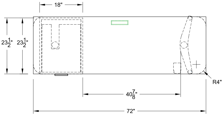
MDL: 42523/A (RECTANGLE) 42503/A (SOFT RECTANGLE) SIZE: 24" X 72"
