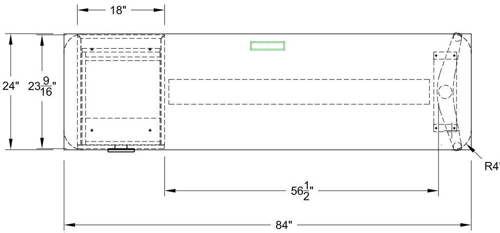
MDL: 42565/F (RECTANGLE) 42545/F (SOFT RECTANGLE) SIZE: 24" X 84"
