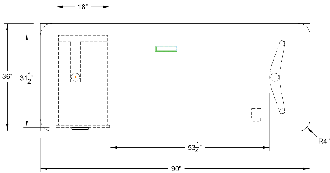
MDL: 42538/A (RECTANGLE) 42518/A (SOFT RECTANGLE) SIZE: 36" X 90"
