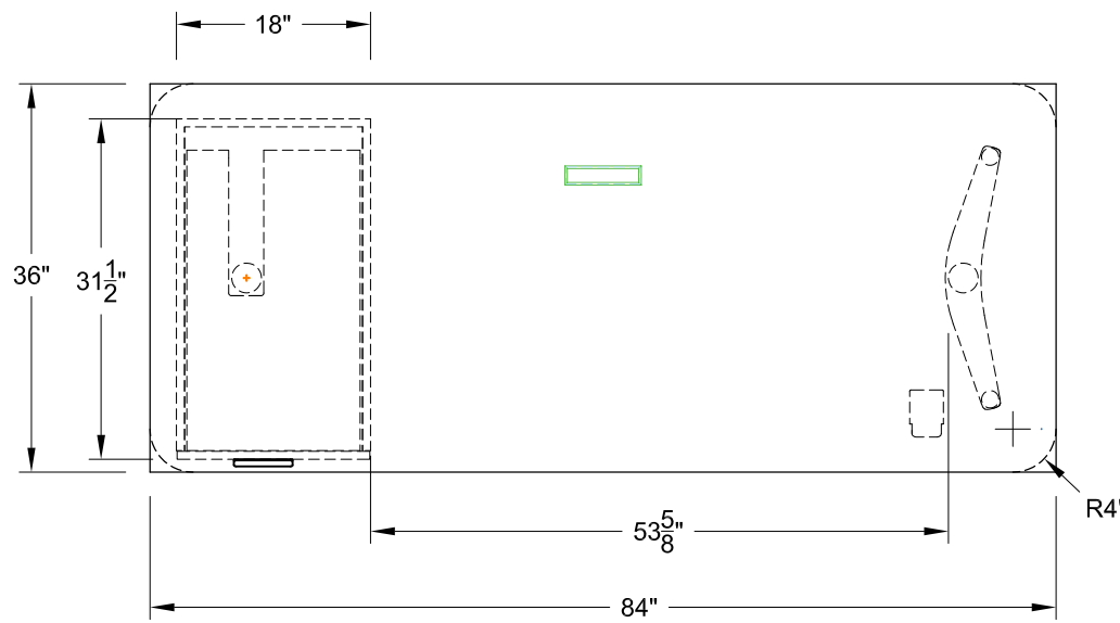
MDL: 42537/A (RECTANGLE) 42517/A (SOFT RECTANGLE) SIZE: 36" X 84"
