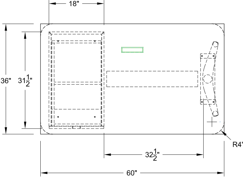
MDL: 42573/F (RECTANGLE) 42553/F (SOFT RECTANGLE) SIZE: 36" X 60"
