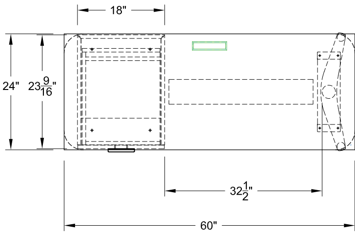
MDL: 42561/F (RECTANGLE) 42541/F (SOFT RECTANGLE) SIZE: 24" X 60"
