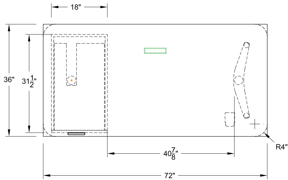
MDL: 42535/A (RECTANGLE) 42515/A (SOFT RECTANGLE) SIZE: 36" X 72"
