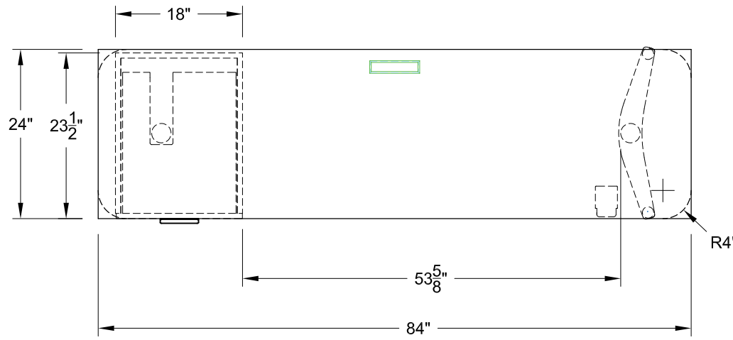
MDL: 42525/A (RECTANGLE) 42505/A (SOFT RECTANGLE) SIZE: 24" X 84"
