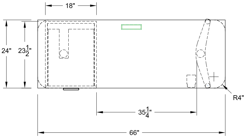
MDL: 42522/A (RECTANGLE) 42502/A (SOFT RECTANGLE) SIZE: 24" X 66"
