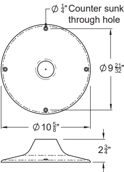
Enlarged Mounting Base Detail
