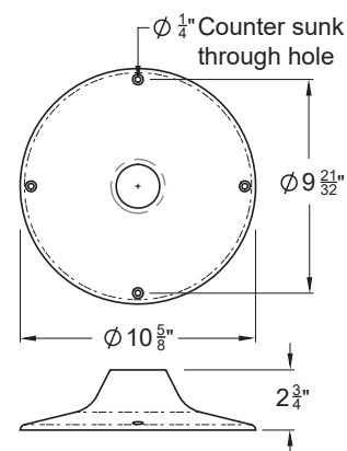
Enlarged Mounting Base Detail
