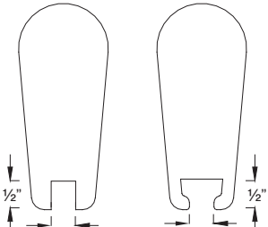
Cable capacity for wood leg
