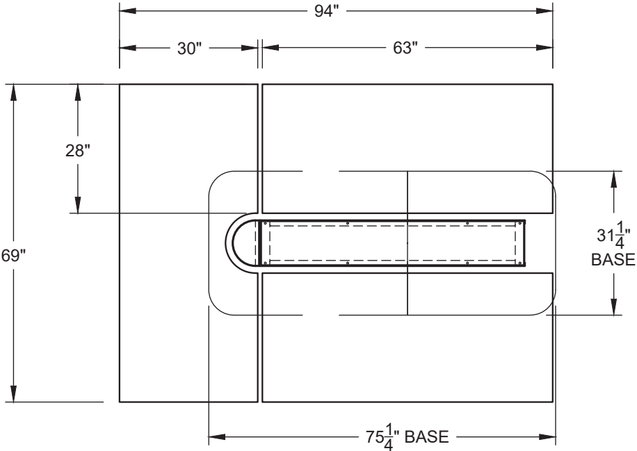
PLAN VIEW
