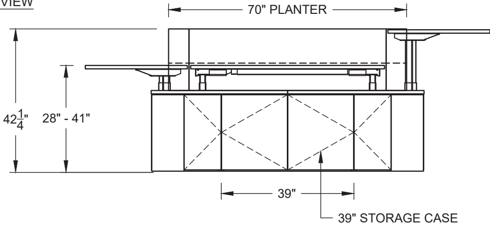
SIDE VIEW
