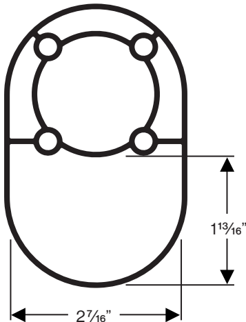
Large capacity post (not to scale)
