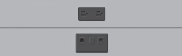
B – 1-Duplex, 2 Data/Voice jacks (2 amp cat 5E RJ 45), 1 Blank position available
