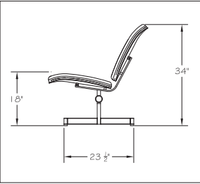
Side elevation
