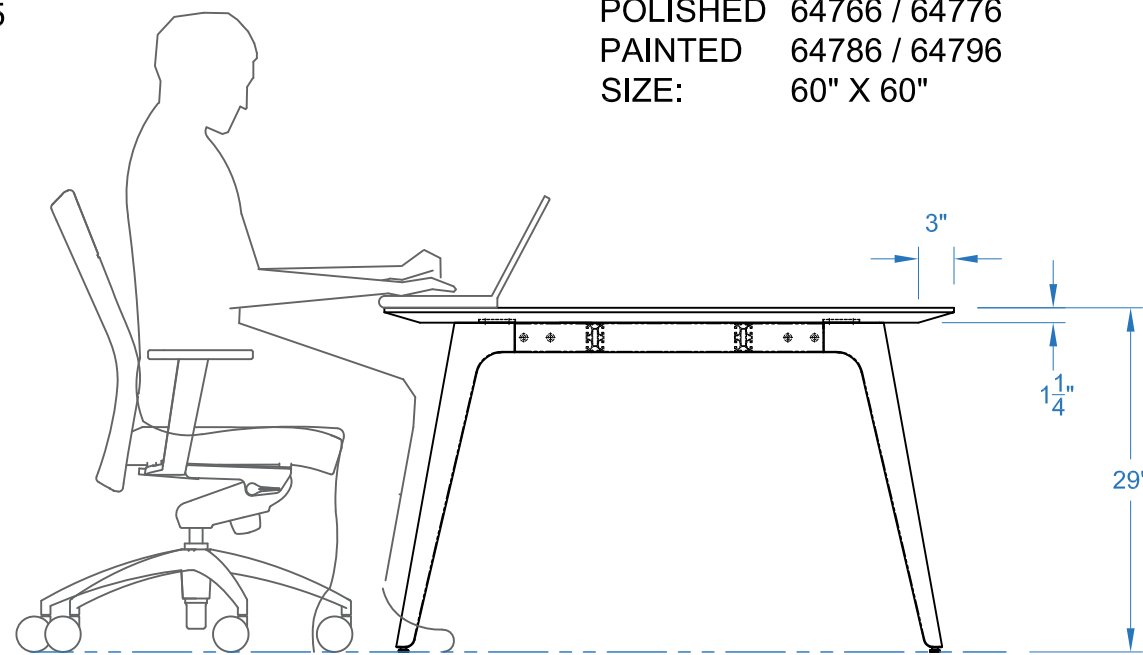
TYPICAL ELEVATION
