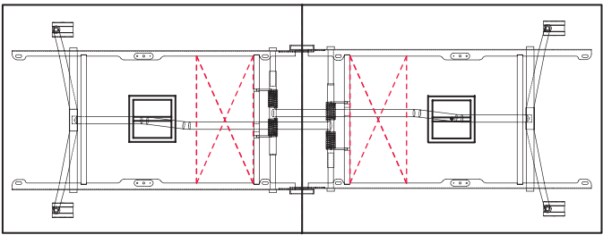
Positioning of Simple Pop Up Forum (Double Sided – Each Side with 4 Ports) on Vox® Folding Table with Solid bases.
