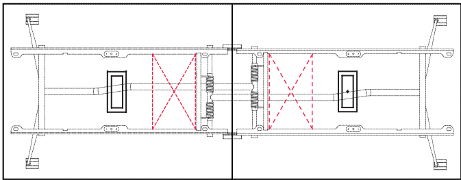
Positioning of Simple Pop Up Forum (Single Sided - 4 Ports) on Vox® Folding Table with Tubular bases.
