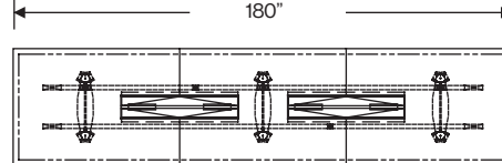
2-troughs - 42"L 4-Simple Forums
