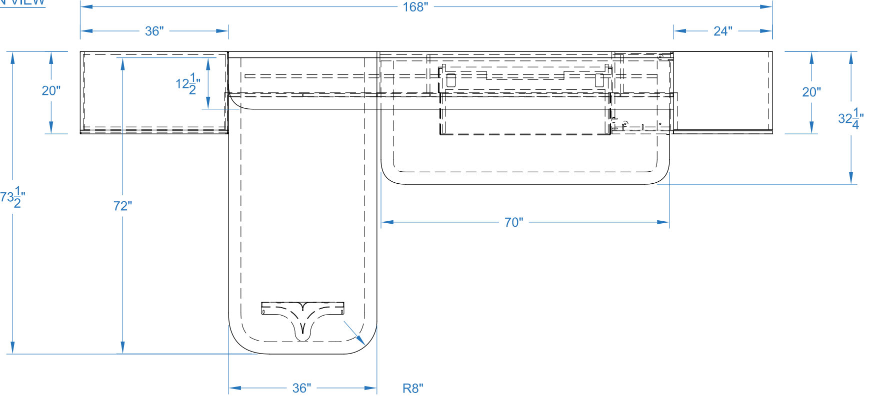
PLAN VIEW
