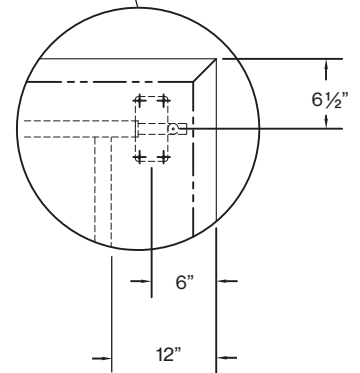
Leg Position Detail
