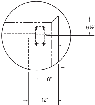
Leg Position Detail
