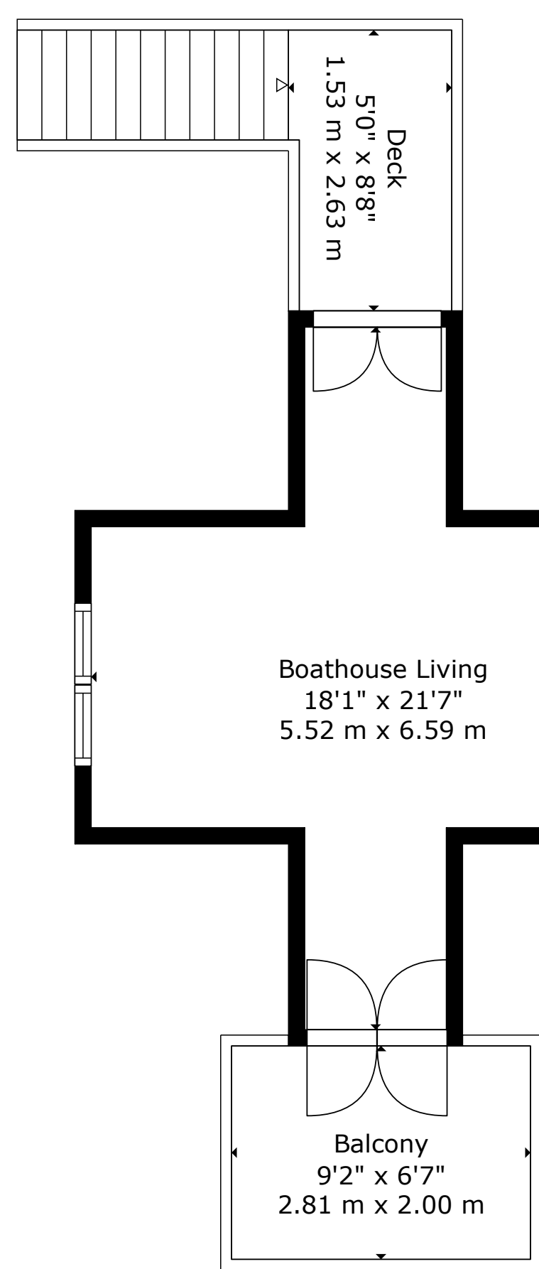
Floor 2
