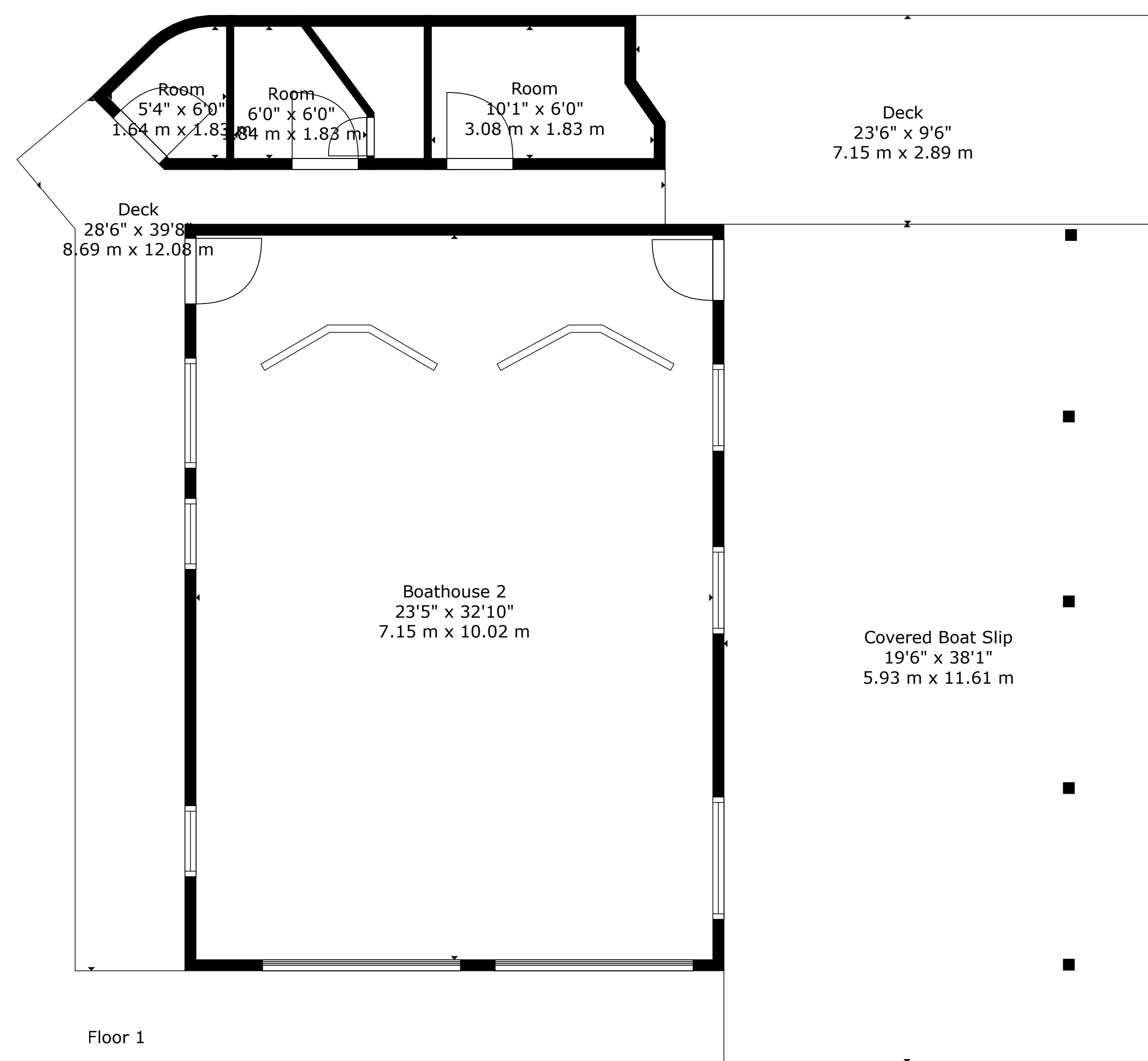
Floor 1
