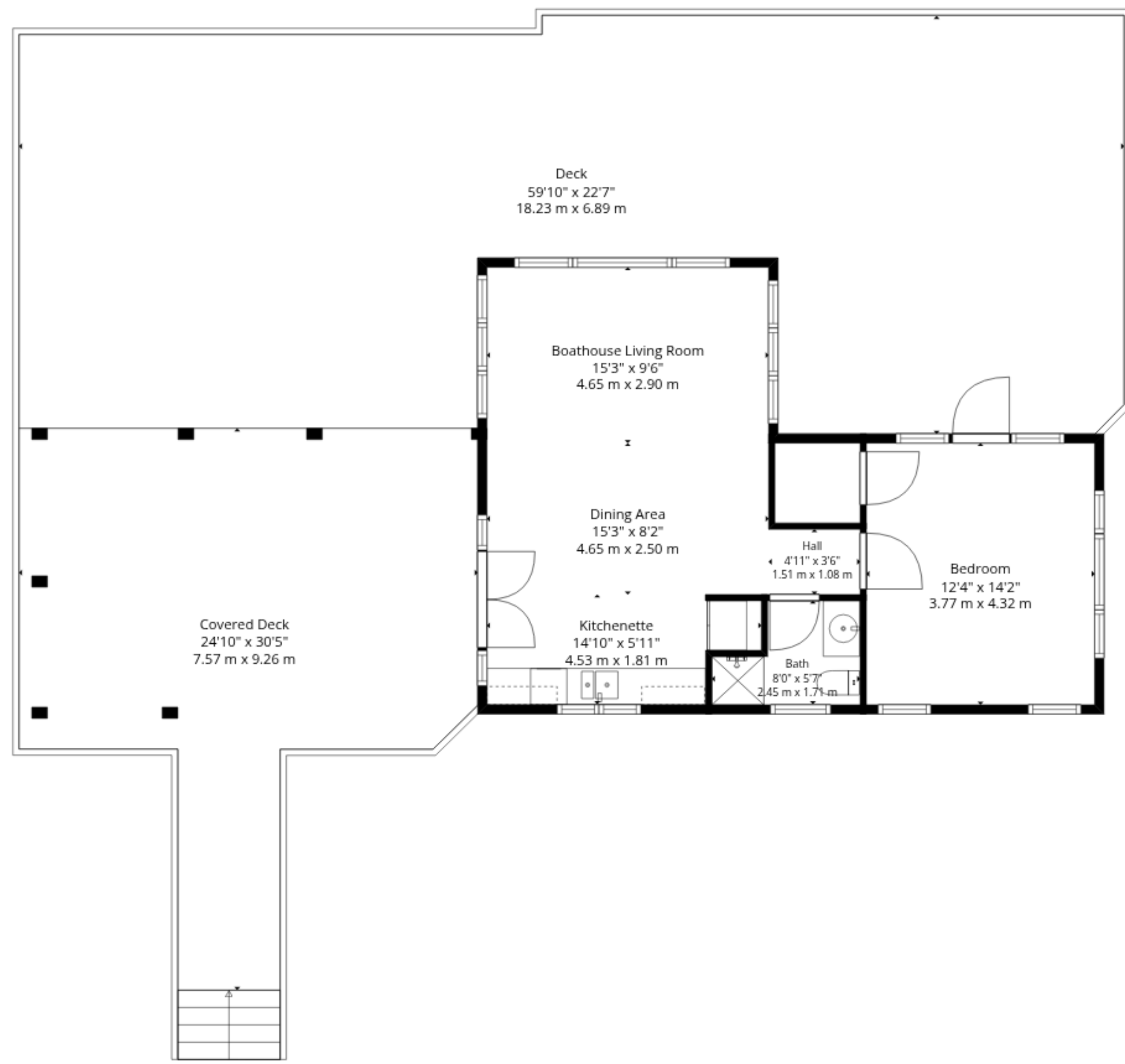
Boathouse Upper Level
