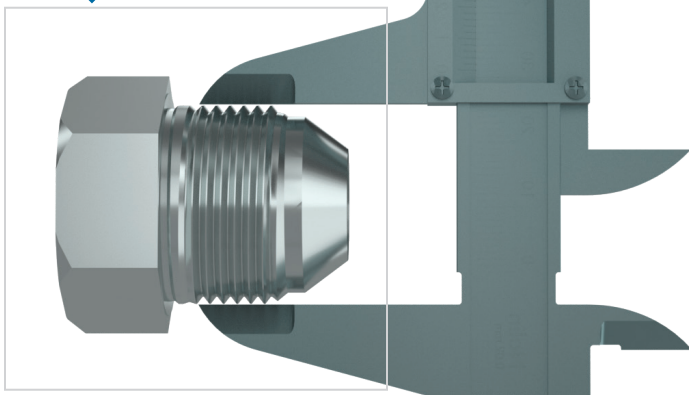
O.D. CALIPER
