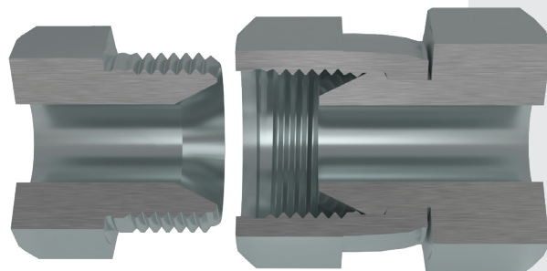
BSPP (parallel)
