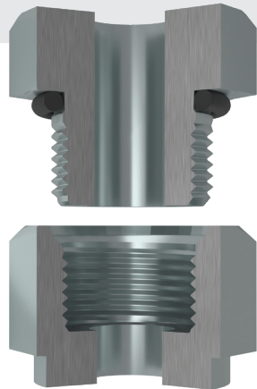
ISO 261 Threads and O-ring Seal
