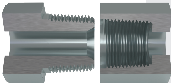
BSPT (tapered)
