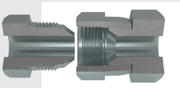
SAE JIC/37°
