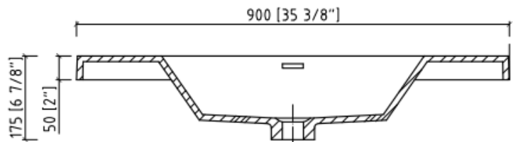
SECTION B-B
