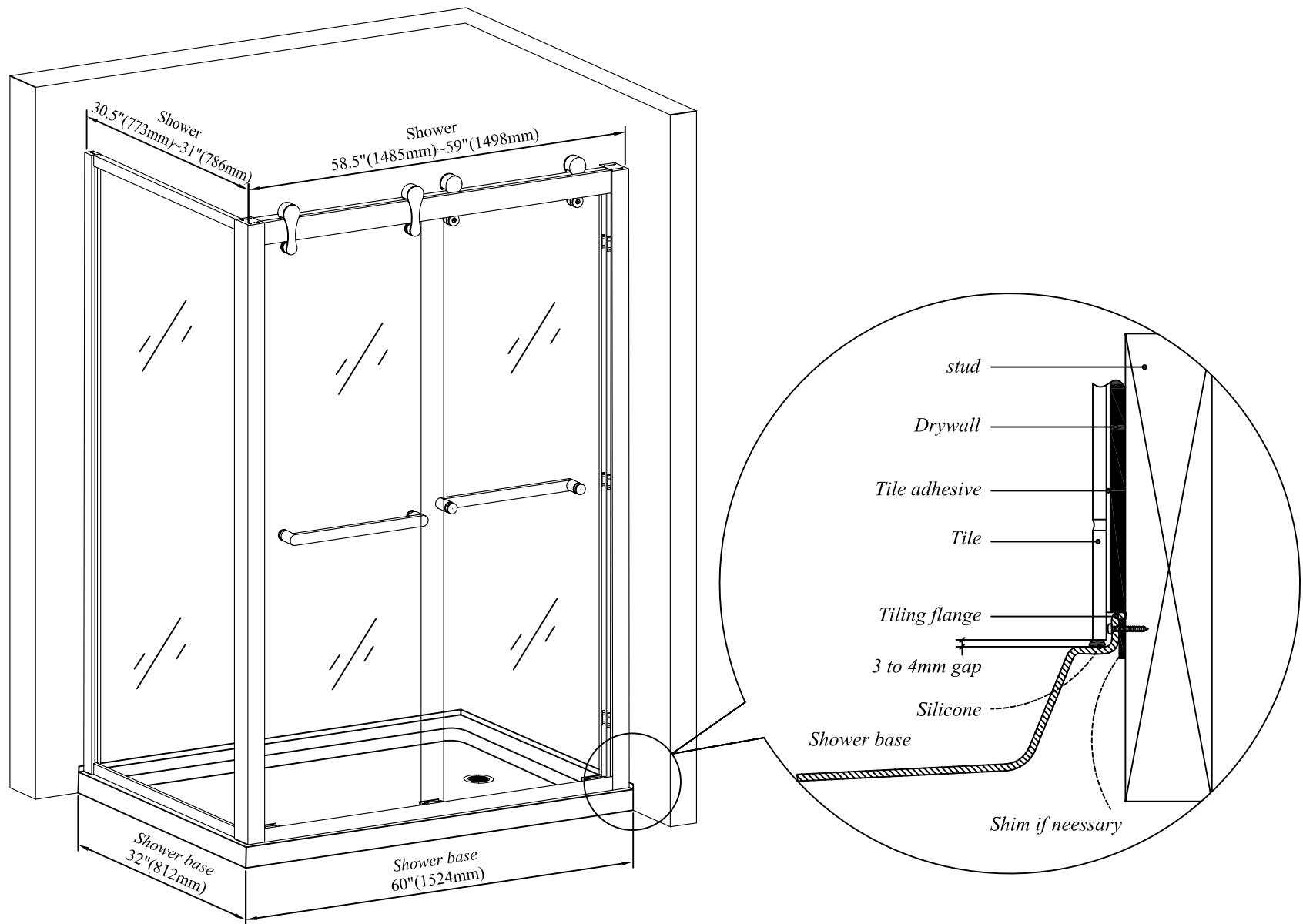
LY3405R-12 60" × 32" × 75" (1524 × 812 × 1900mm)
