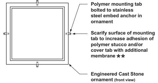
FIGURE 6 ANCHOR TAB FOR E.I.F.S. DETAIL
