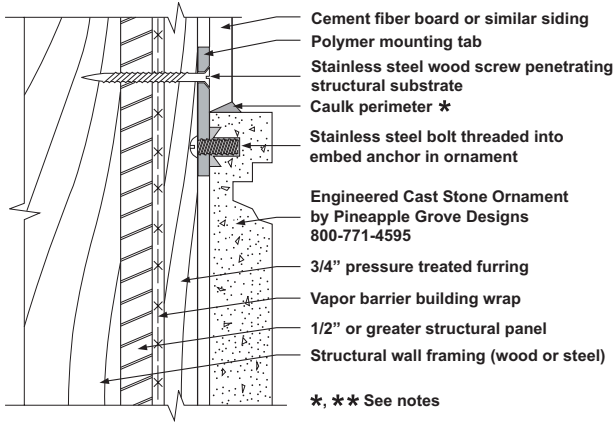
FIGURE 10 MOUNTING TAB FOR FRAME CONSTRUCTION
