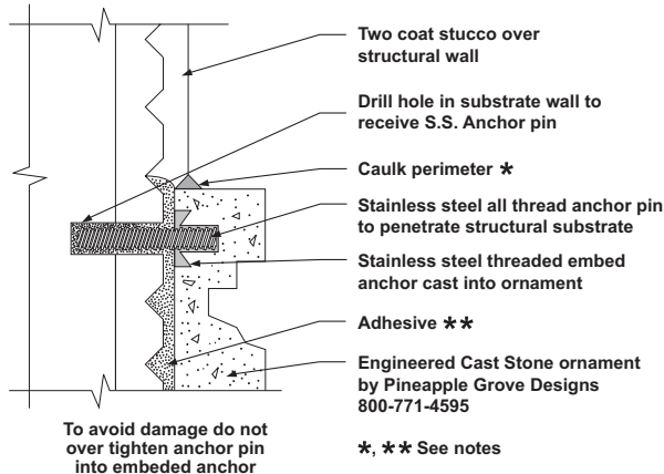
FIGURE 9 ANCHOR DETAIL
