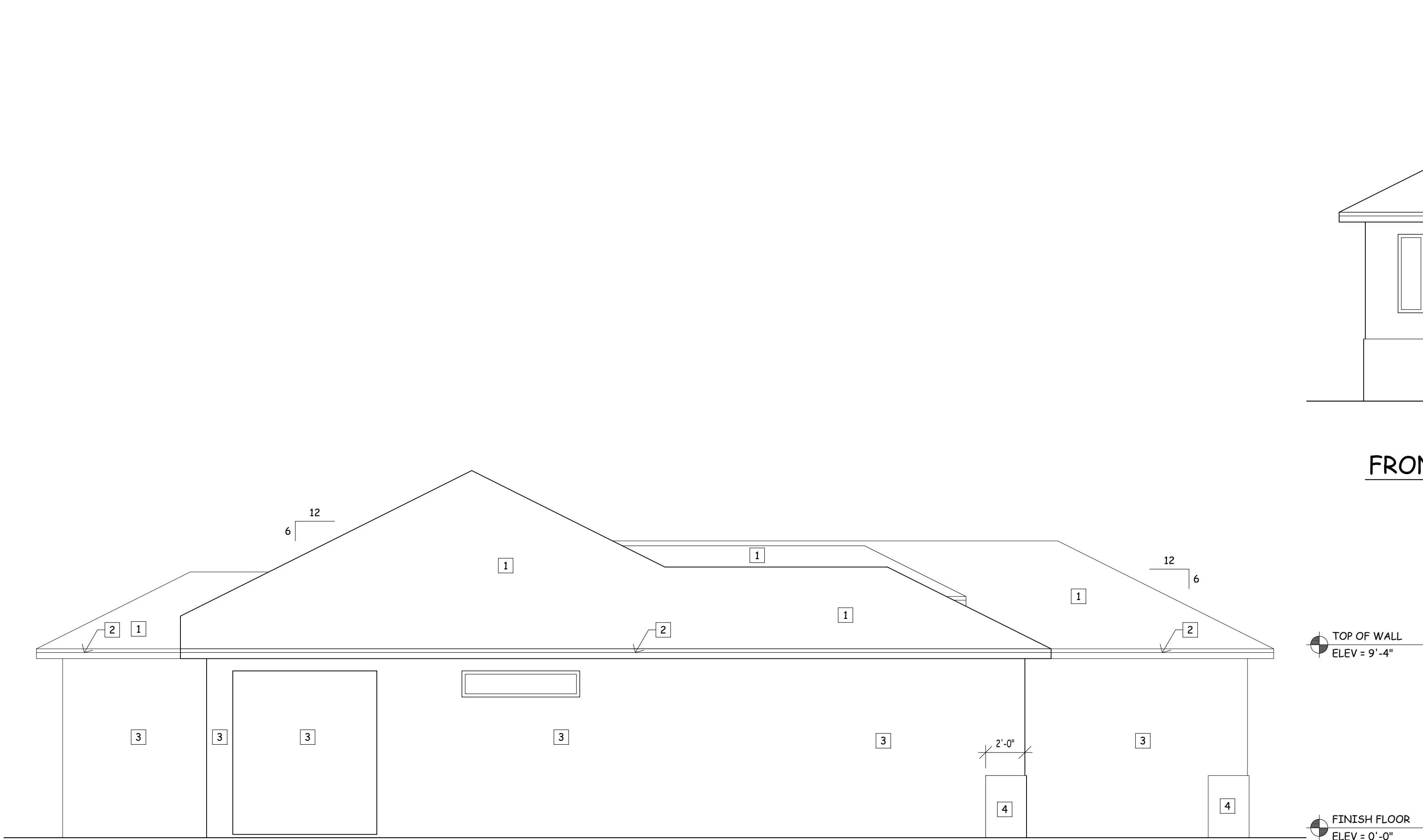
LEFT ELEVATION
