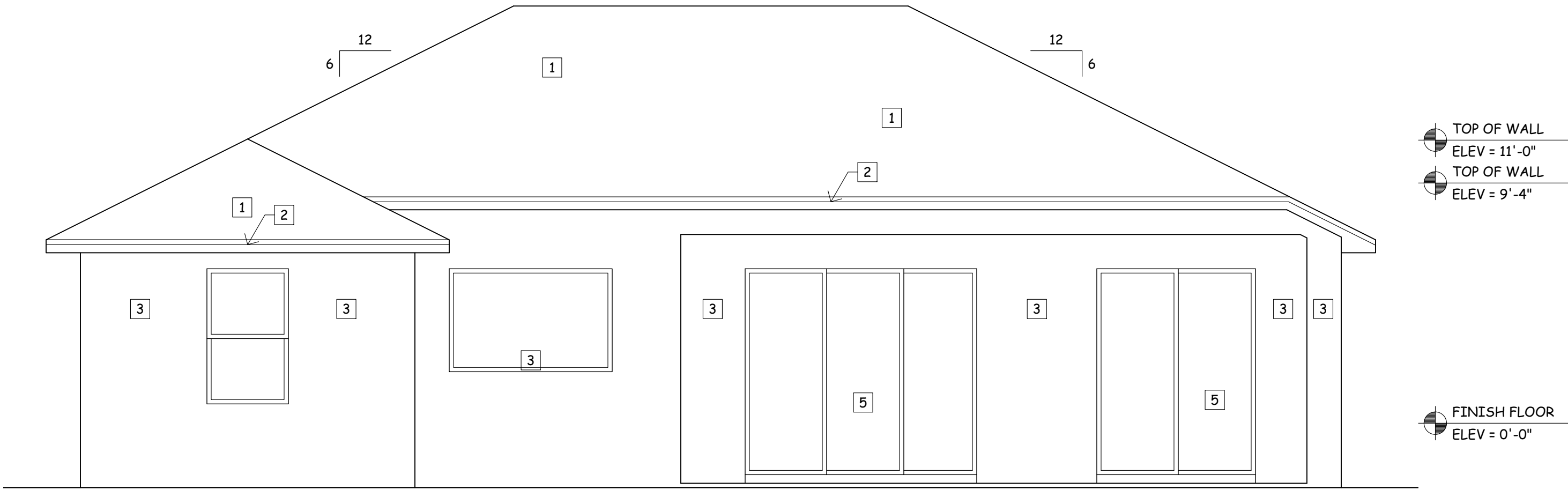
BACK ELEVATION
