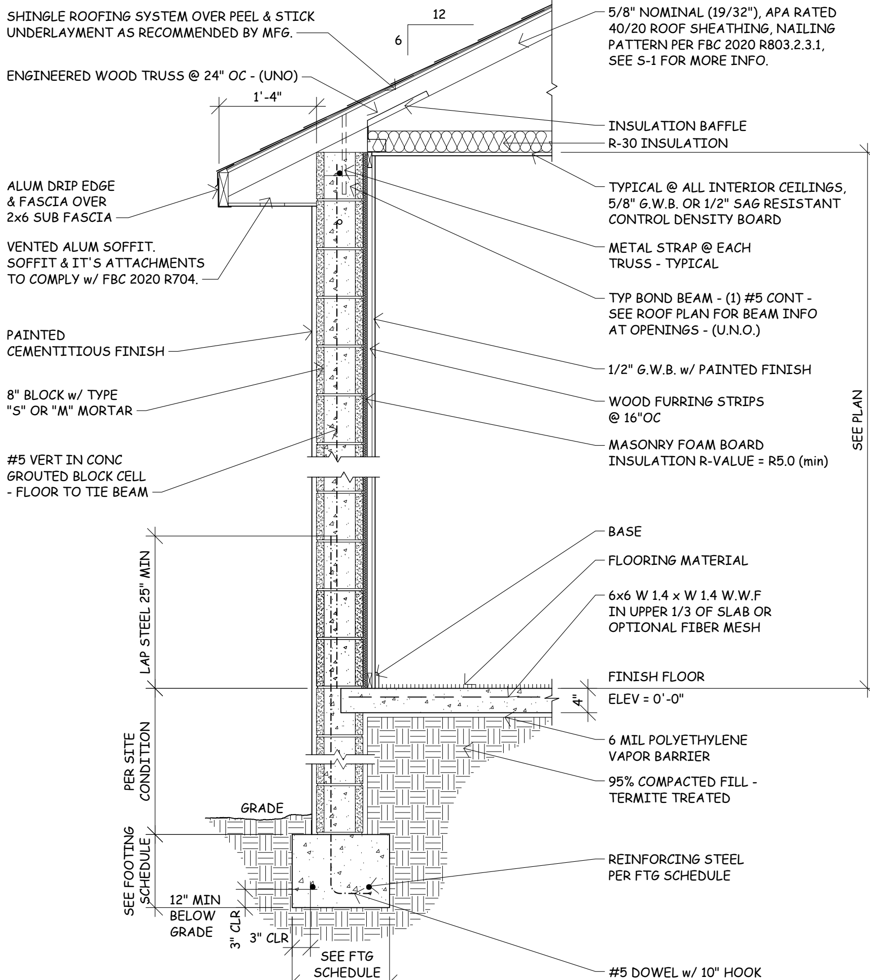
TYPICAL WALL SECTION
