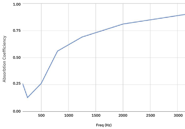
Absorbtion Coefficiency vs. Freq (Hz)
