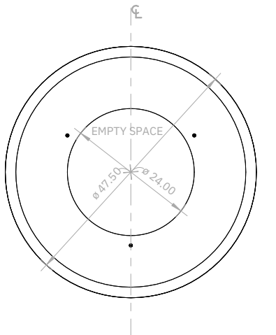
3 PLAN VIEW - MIDDLE DONUT 3/4" = 1'-0"
