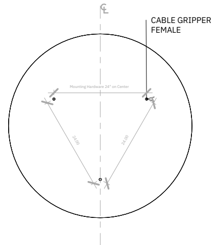
4 PLAN VIEW - TOP 3/4" = 1'-0"
