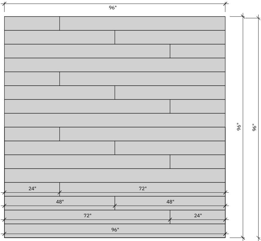
1 SUBWAY TILE - (2) STARTER KITS - ELEVATION PANEL SIZE & QUANTITY • 24" x 6" Qty. 8 • 48" x 6" Qty. 8 • 72" x 6" Qty. 8 • 96" x 6" Qty. 4
