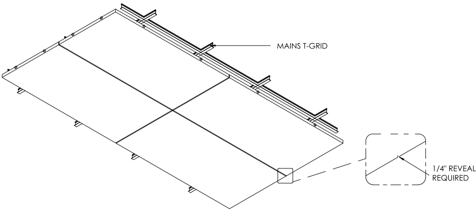
1 TRAVA w/ HOOK & SADDLE CLIP - BOTTOM DIMETRIC
