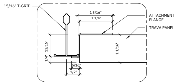
3 ATTACHMENT DETAIL
