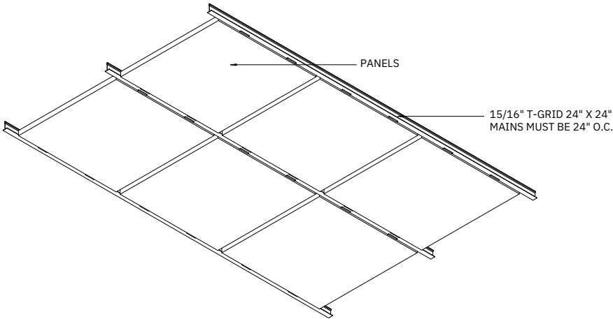
3 TRAVA REGULAR ASSEMBLY - BOTTOM DIMETRIC
