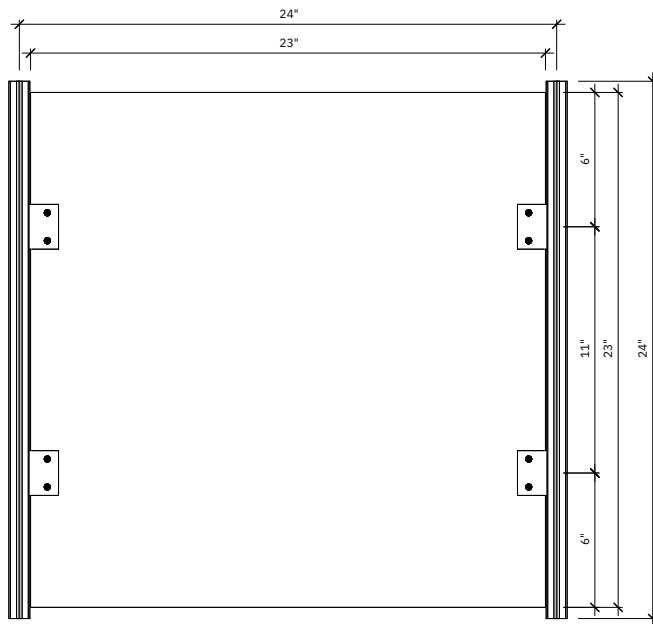
1 TRAVA TEGULAR - PLAN VIEW
