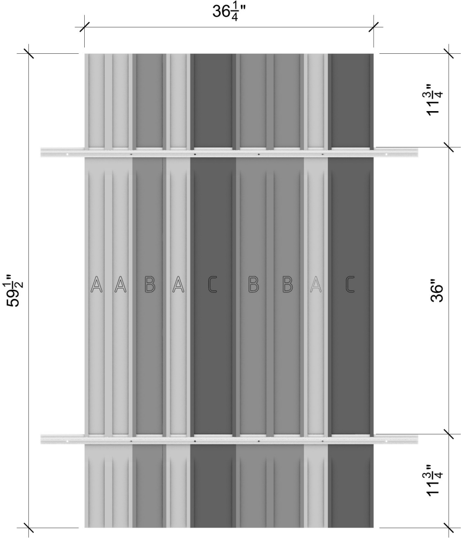
1 BACK VIEW SCALE 1:12
