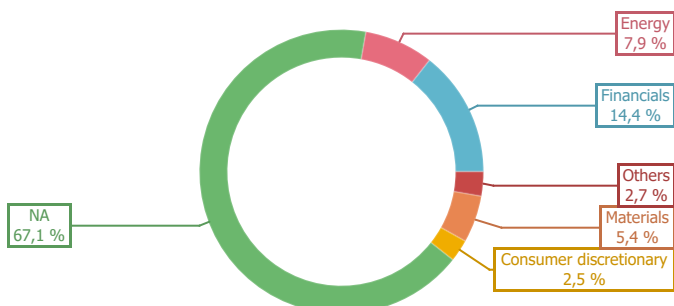
Sector Allocation
