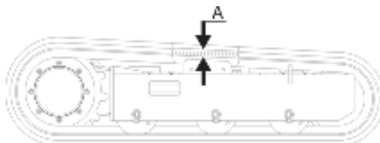
Fig. 160 Controle spanning rupsband 2
