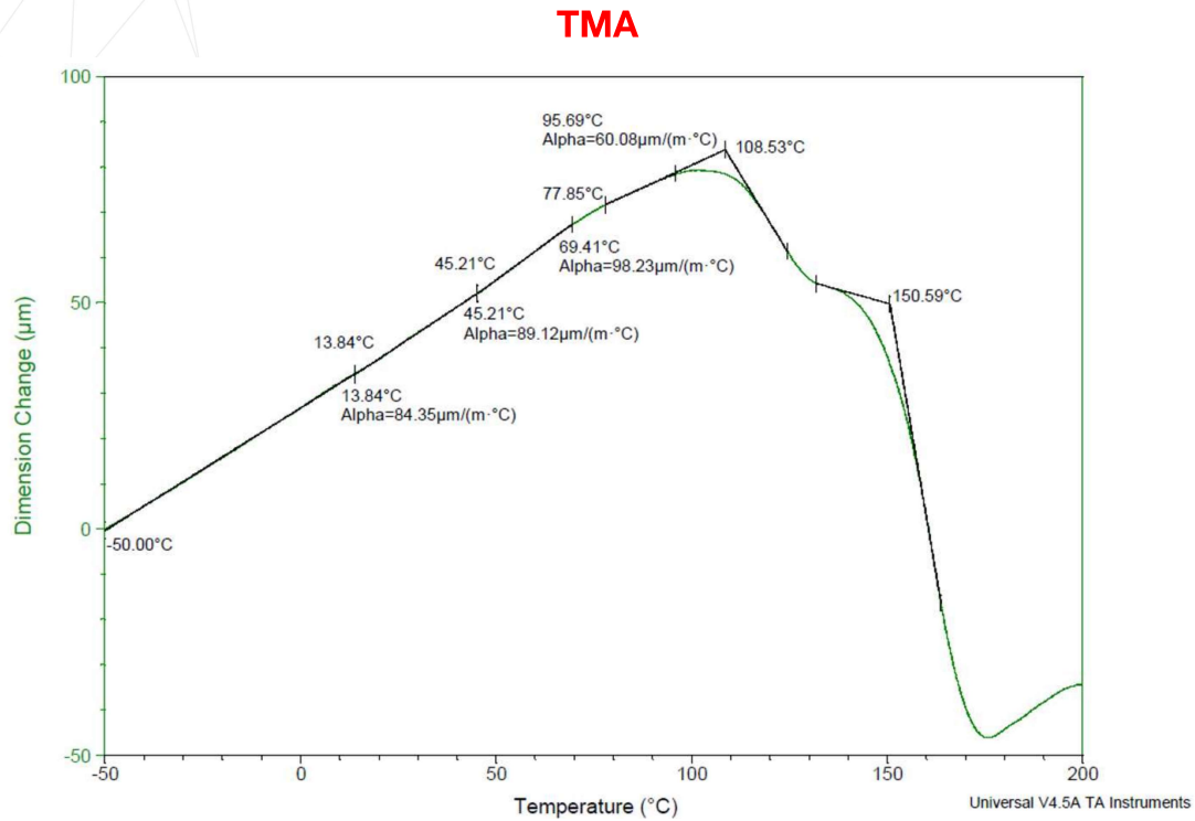
Figure 2. Dimension change data as a function of temperature for the Nylon 12 Flat (XY) sample.
