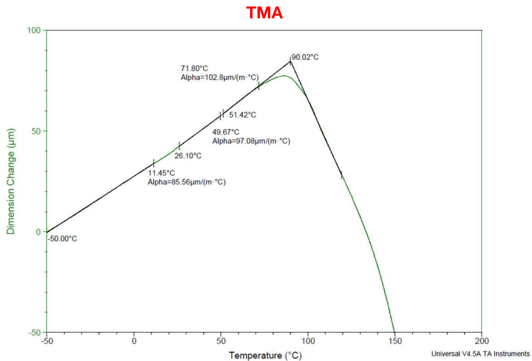
Figure 3. Dimension change data as a function of temperature for the Nylon 12 On Edge (XZ) sample.
