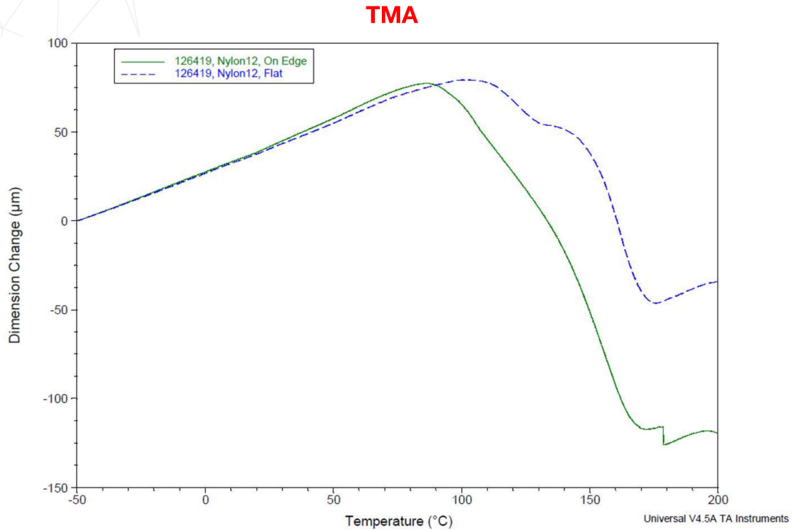
Figure 4. Overlay of the dimension change data for the Flat (XY) and On Edge (XZ) Nylon 12 samples.
