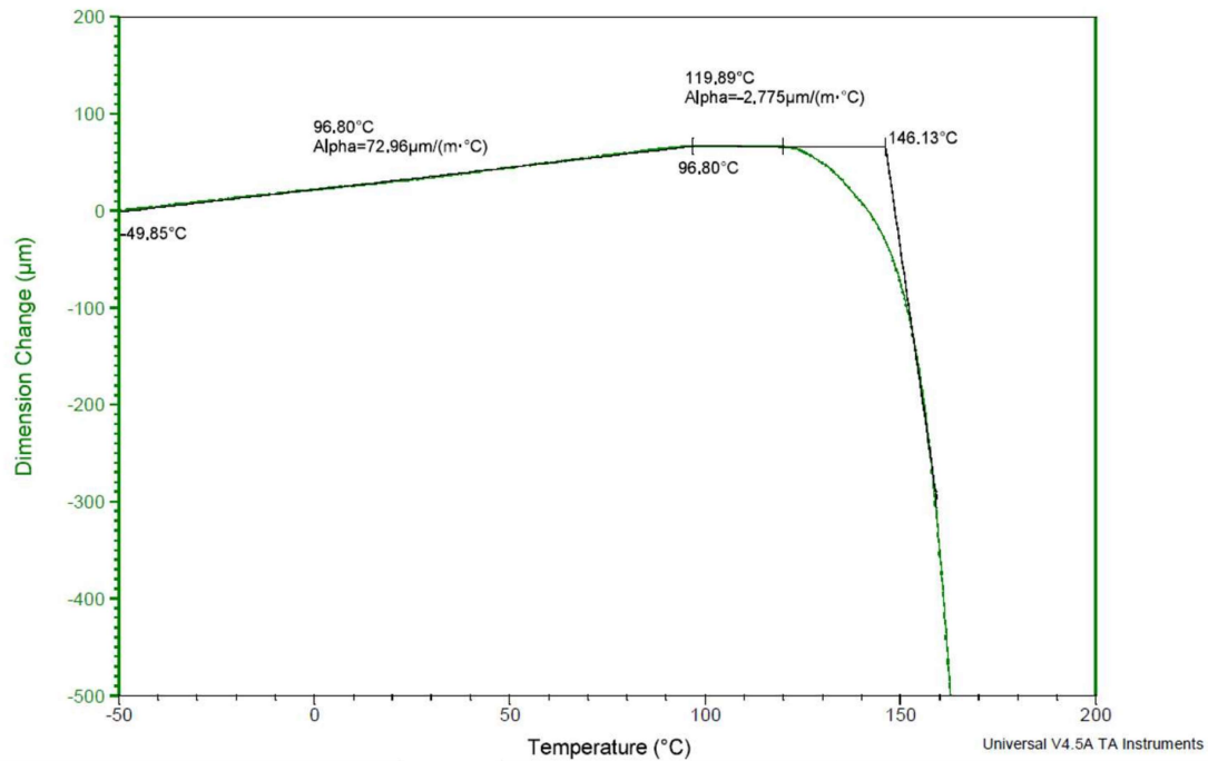
Figure 3. Dimension change data as a function of temperature for the PC-ABS On Edge (XZ) sample.
