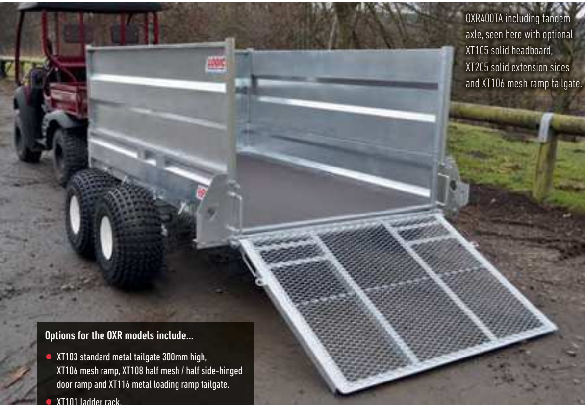
Strong monocoque construction with rope hooks and high quality galvanising for long life protection.
