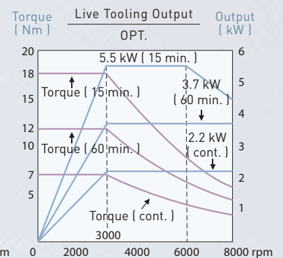
12-station live tooling turret
