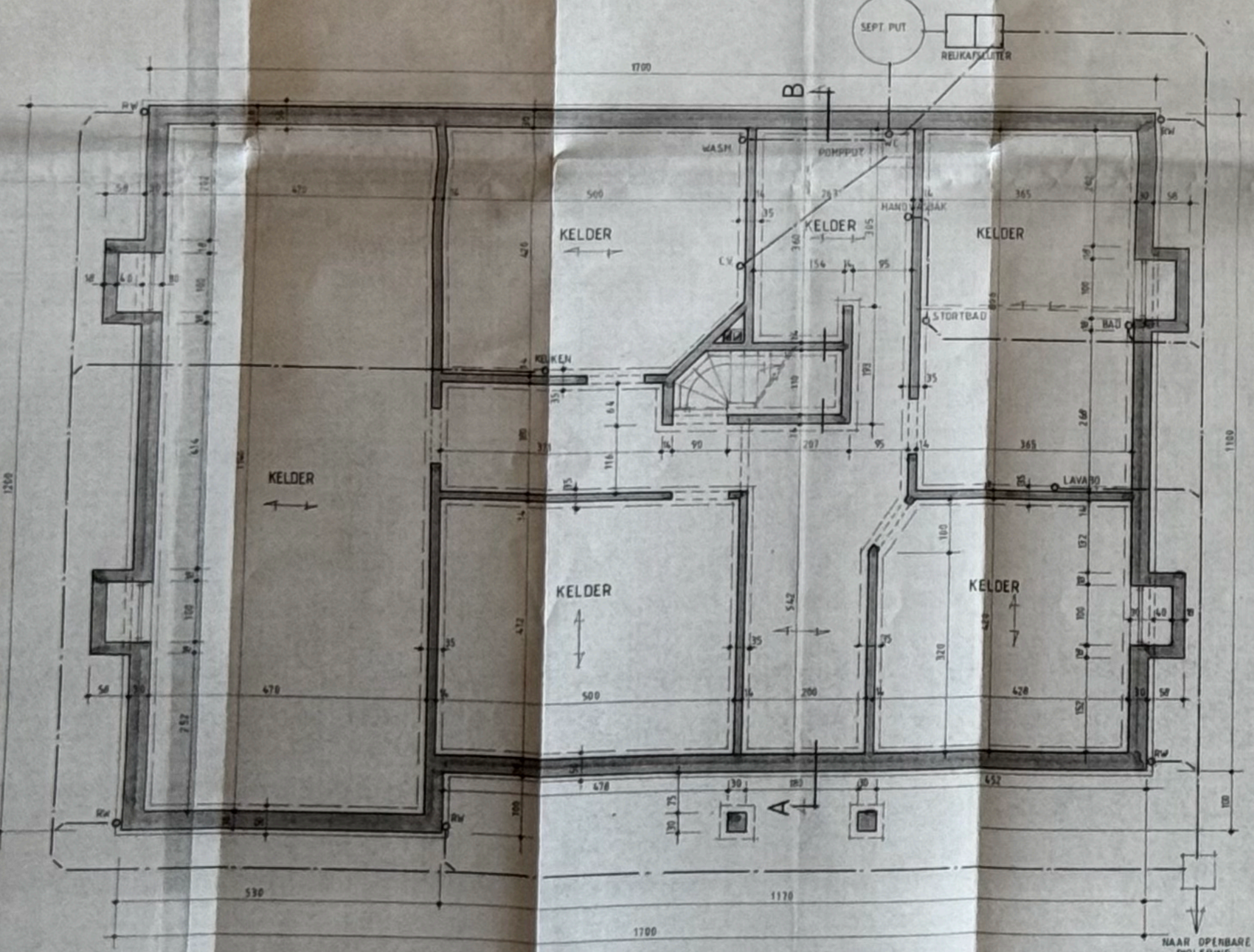
KELDER - FUNDERING - RIOLERING
