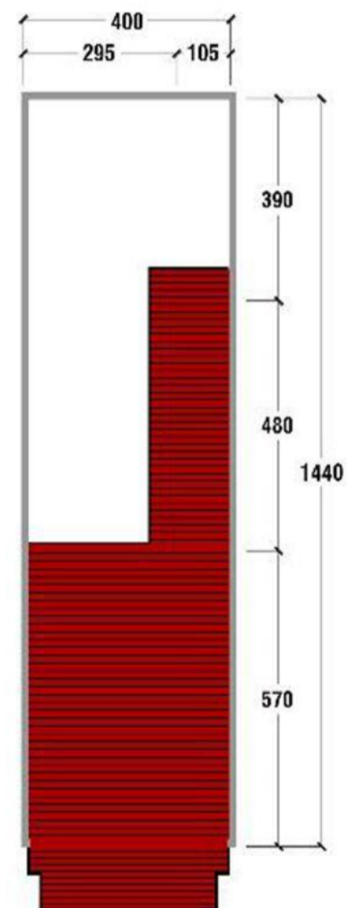
LANTAI ATAP
