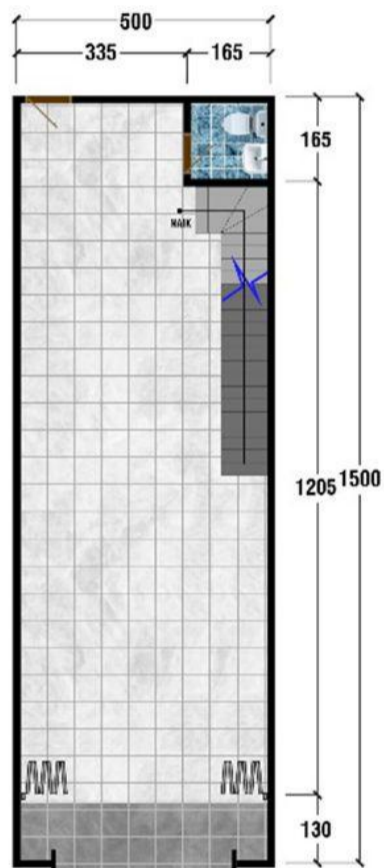
LANTAI 1
