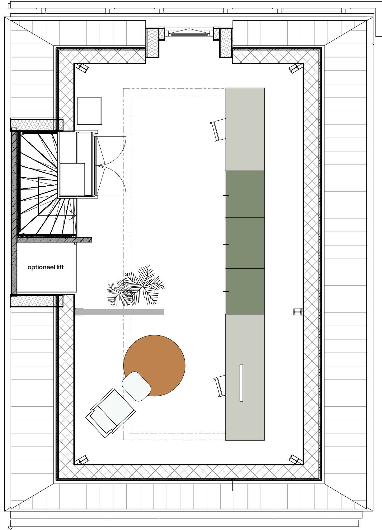
2 o verdieping BWNR 09
