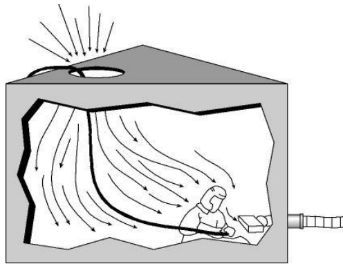
Local Exhaust Ventilation (Wiley, 2005)
