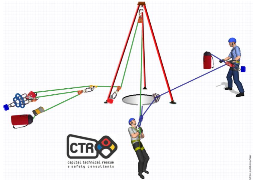
Hauling with a Change of Direction on Main Line - Tripod Hobbles Omitted for Clarity
