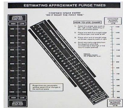
Air Systems International Manual, blower capacity plate, and nomograph.
