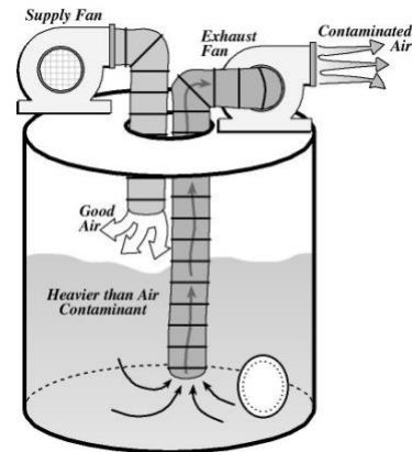
Push / Pull Ventilation (Wiley, 2005)
