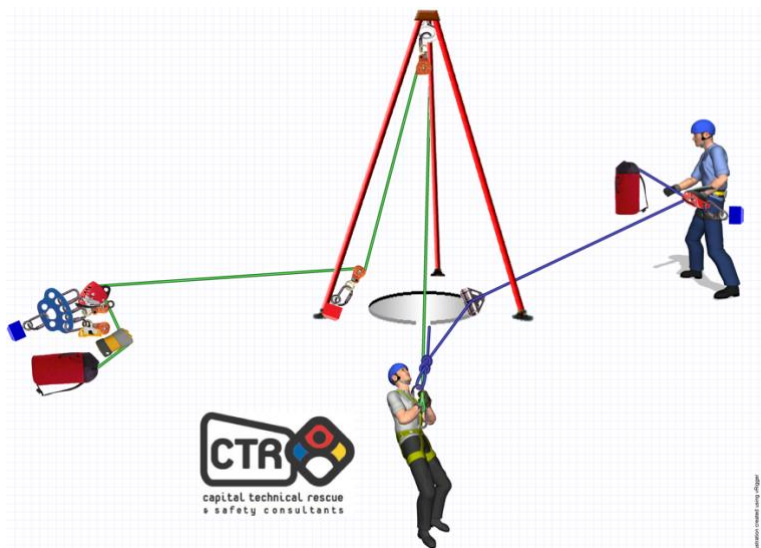
Lowering with a Change of Direction - Tripod Hobbles Omitted for Clarity
