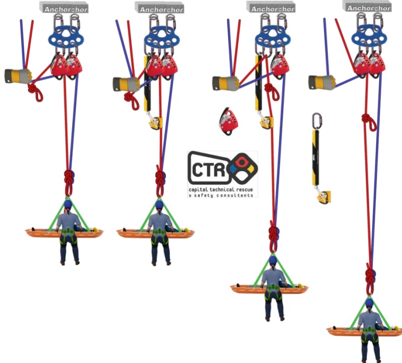
Dual Main "UP" Knot Pass w/ Petzl ASAP
