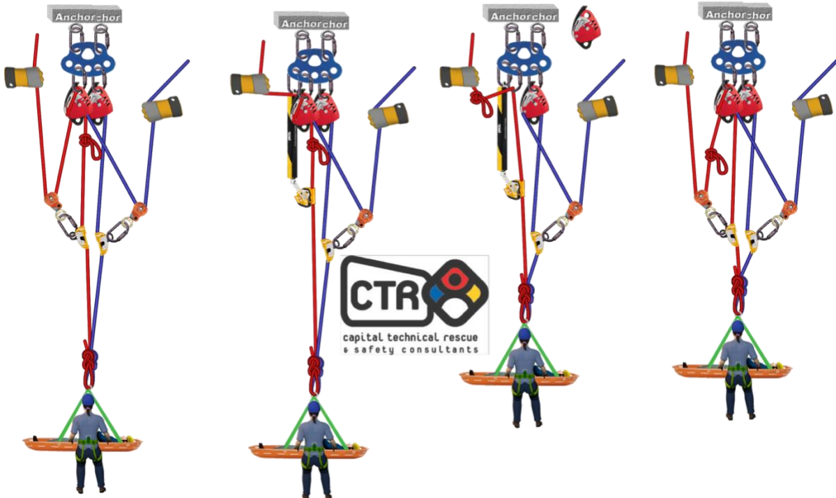
Dual Main "UP" Knot Pass w/ Petzl ASAP
