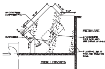
2 DUMPSTER PAD PLAN
