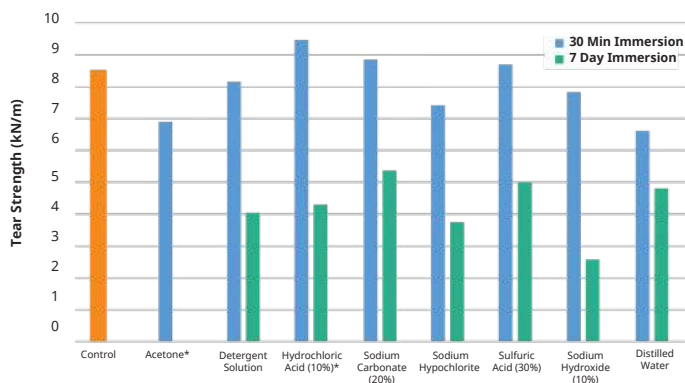
FIGURE 4 RUBBER-65A BLK
