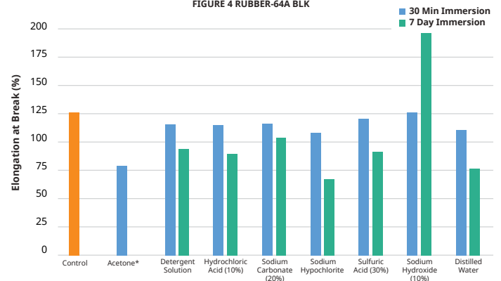
FIGURE 4 RUBBER-64A BLK
