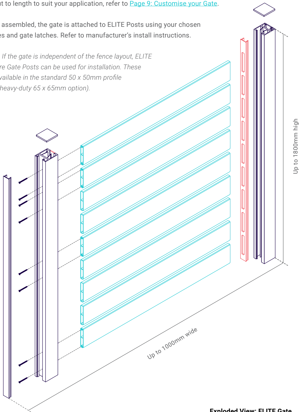
Exploded View: ELITE Gate
