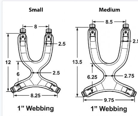
COMFORTFIT TRIM – 30618 / 30619
