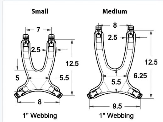
COMFORTFIT FULL – 30589 / 30590
