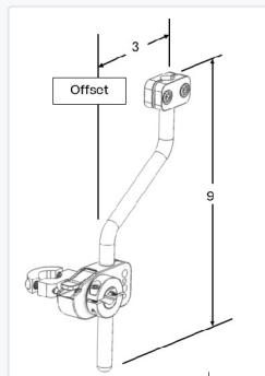
30248 – SHORT ARM
