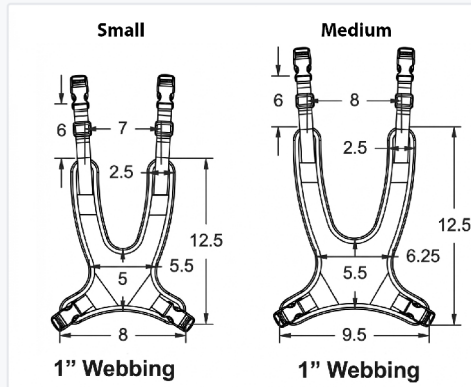
EXT. STRAPS FULL – 30594 / 30595
