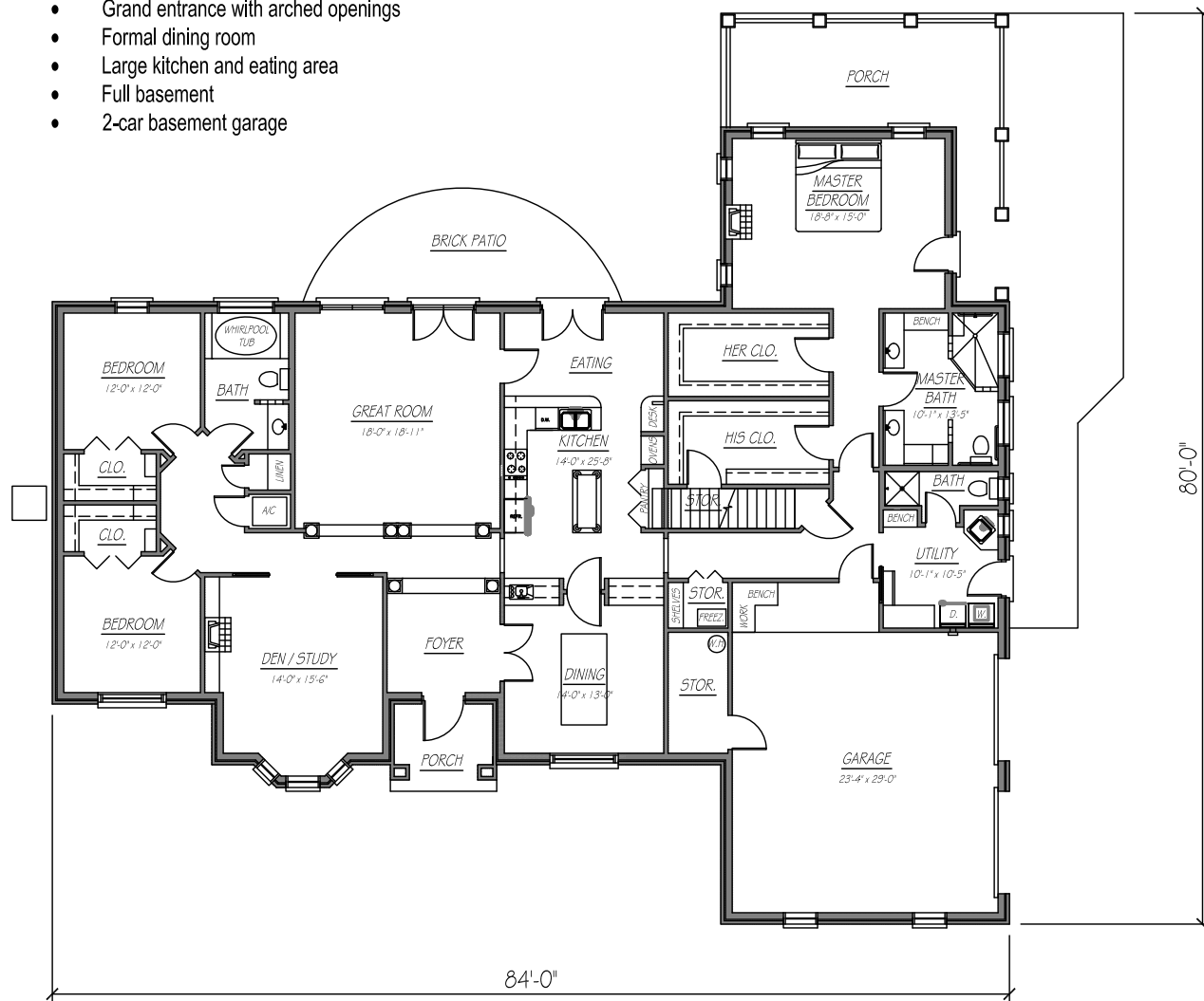
MAIN LEVEL
