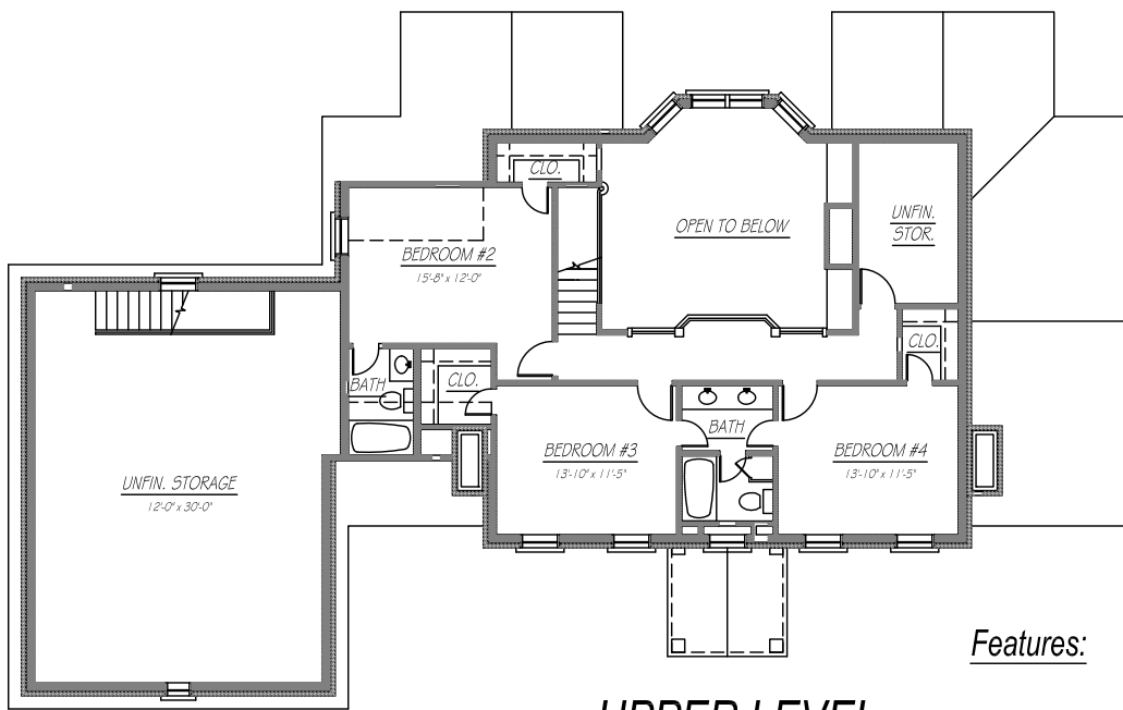
UPPER LEVEL
