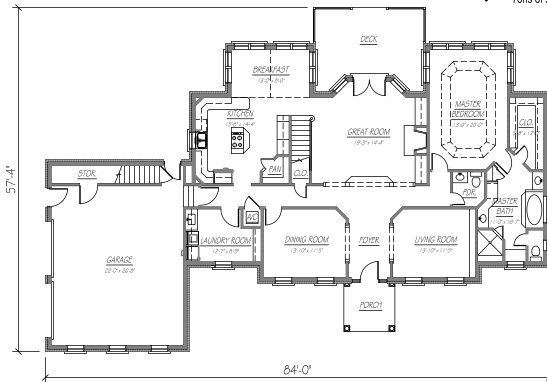
MAIN LEVEL
