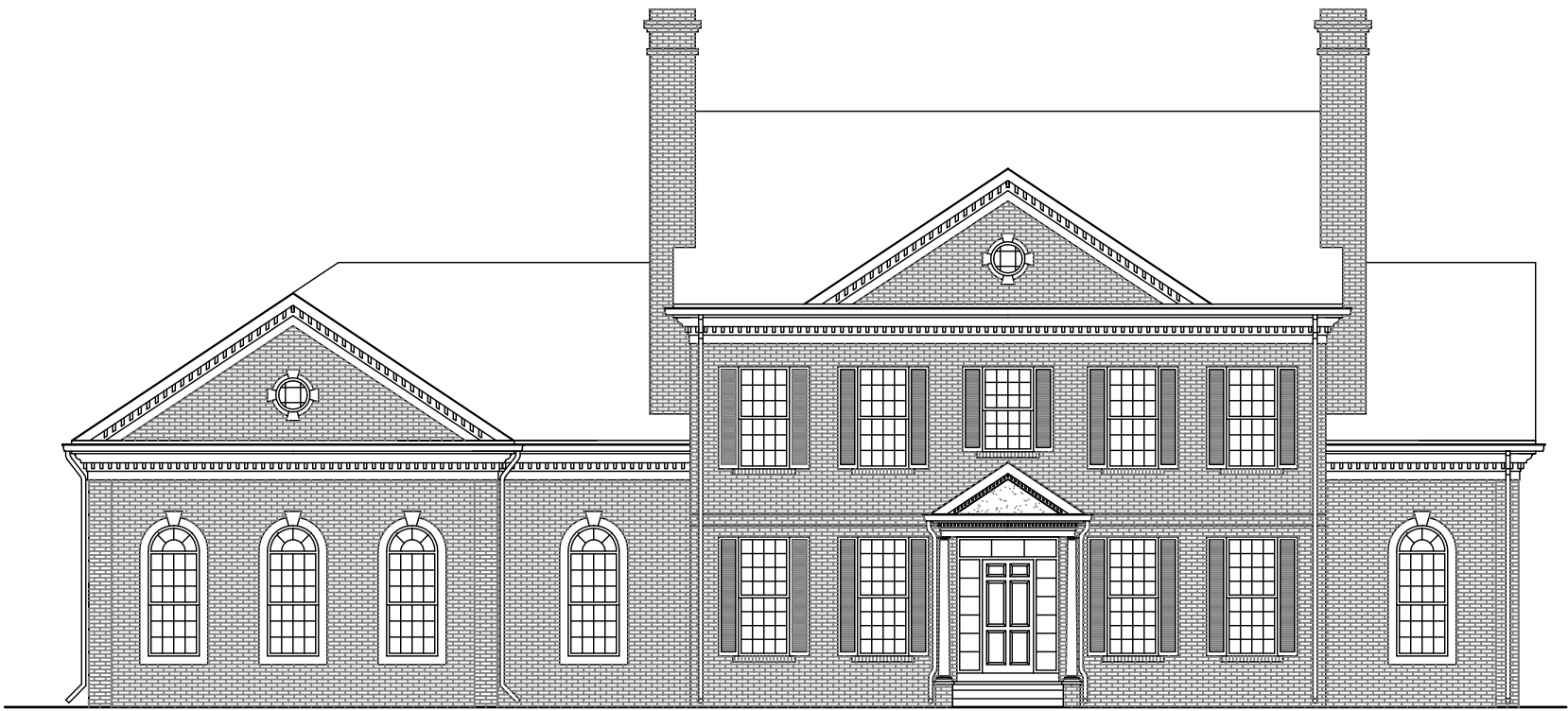
FRONT ELEVATION
