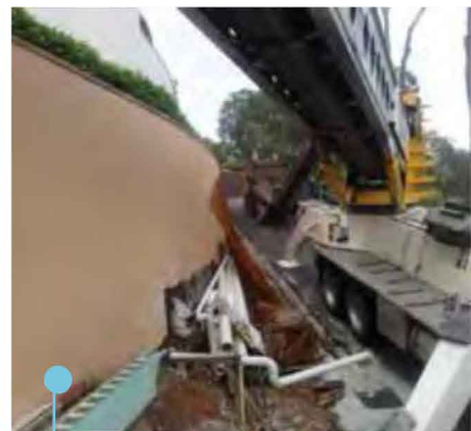
Flexible options for positioning outriggers allow this Telebelt to set up in an area with restricted access.
