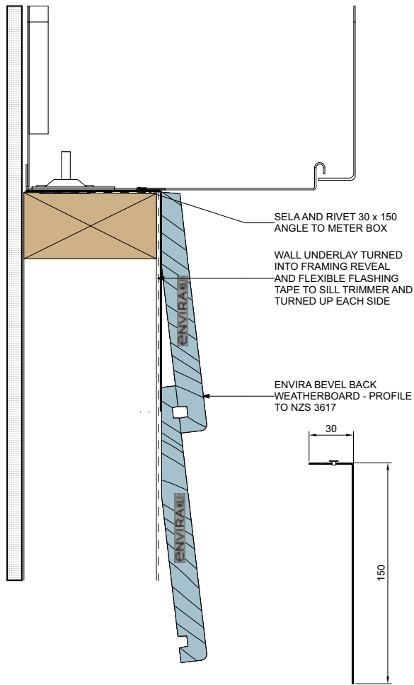
FLASHING DIMENSIONS
