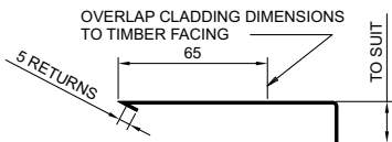
FLASHING DIMENSIONS
