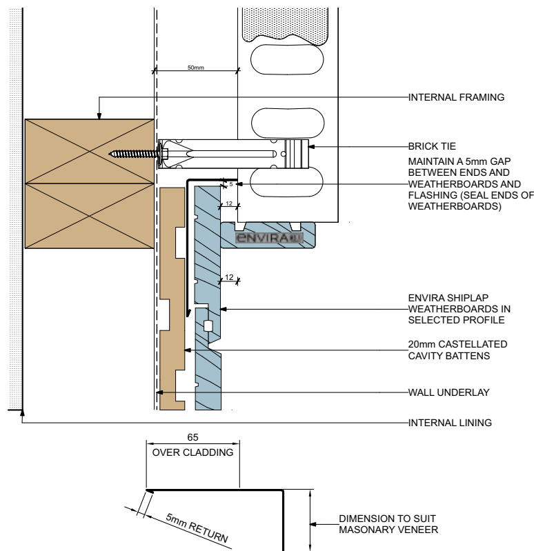
FLASHING DIMENSIONS
