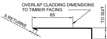
FLASHING DIMENSIONS
