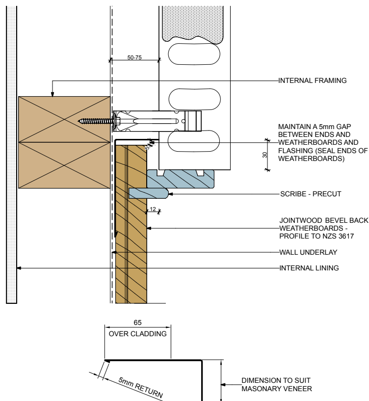
FLASHING DIMENSIONS
