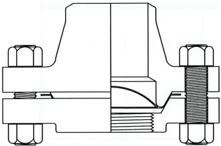
RDH-3 (Threaded Inlet/Welded Outlet)
