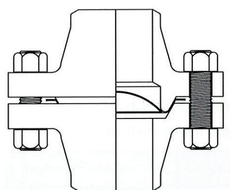
RDH-6 (Welded Inlet/Welded Outlet)
