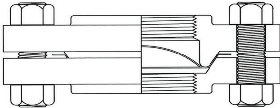
RDH-1 (Threaded Inlet/Flat Outlet)
