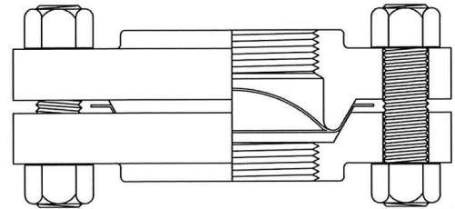
RDH-2 (Threaded Inlet/Threaded Outlet)
