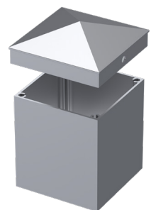
Exposed Cap (on 90 x 90mm post) Code: PC90AL
