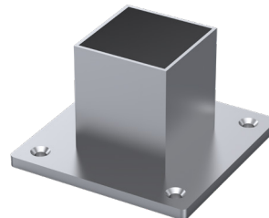
160 x 160mm Welded flanged base (90 x 90mm post) 90x90 x 1250mm - FP90125EB 90x90 x 1550mm - FP90155EB 90x90x 1850mm - FP90185EB
