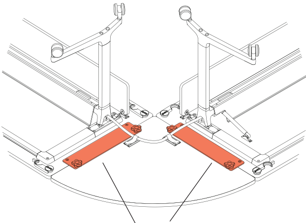
Joining Plates
